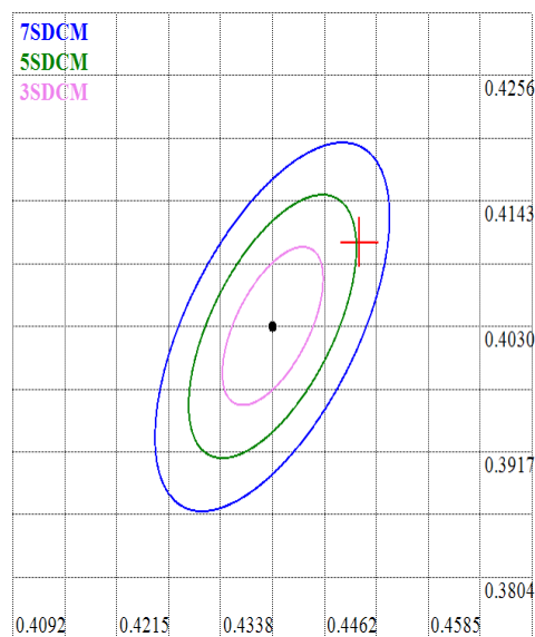
Nominal CCT: ANSI_F3000K x0=0.4503 y0=0.4106
